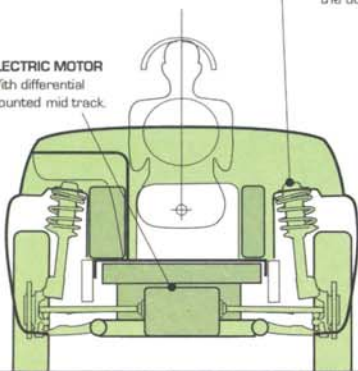
SECTION thru FRONT SPINDLE
