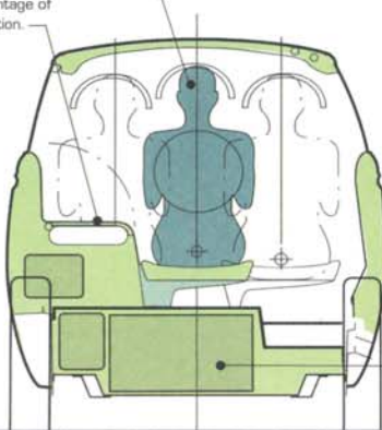
SECTION thru DRIVER
